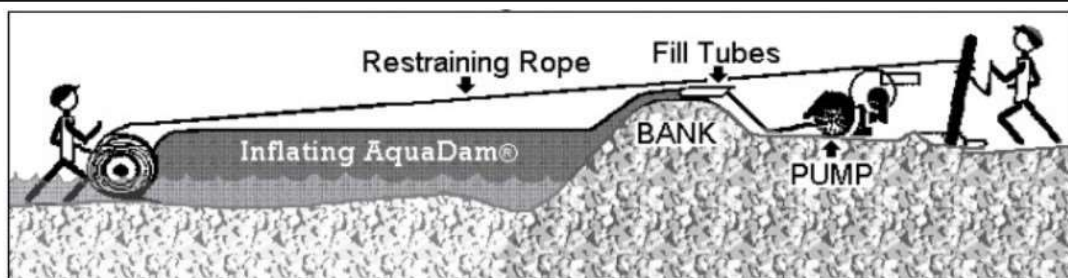
Figure 4. A cross section of a large AquaDam being installed in flowing water, illustrating the location of the berm, pumps, ropes, laborers and the inside water head pressure, compared to the outside water levels.
